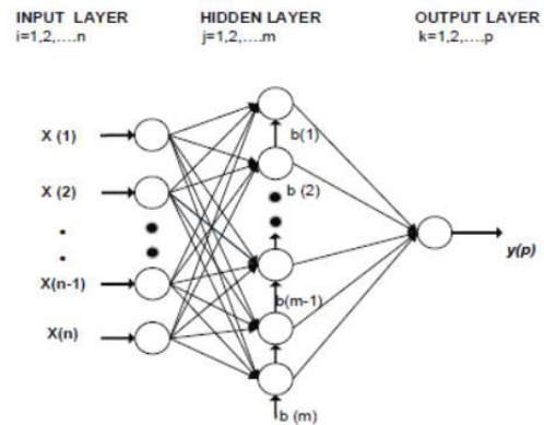
Fig. 4. An ANN model with a single hidden layer
