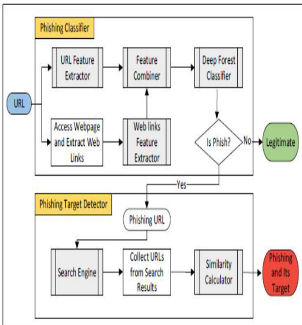
Fig. 3. Overview of the proposed work
