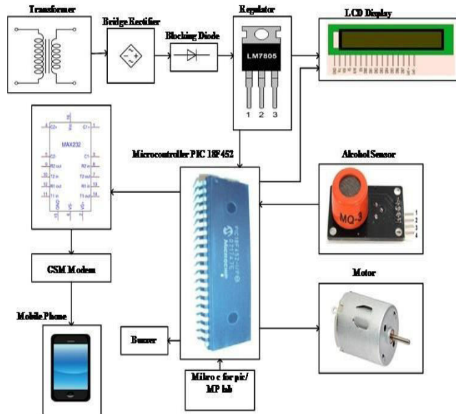
Fig. Architecture of the System
