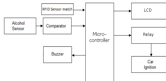
Fig. Block Diagram of the System
