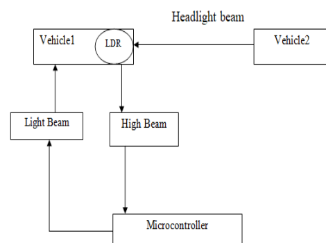
Figure 6. Block Diagram
