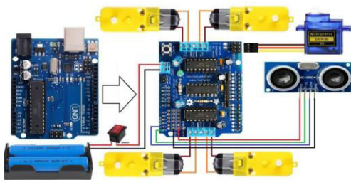
Figure 3. Circuit diagram of anti collision
