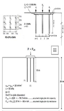
Fig. 15. Definition of hypothetical example by Poulos [1] which is used for software validation.
