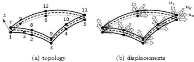
Fig. 6. Schematic of Line interface components for connecting beam part to solid element.
