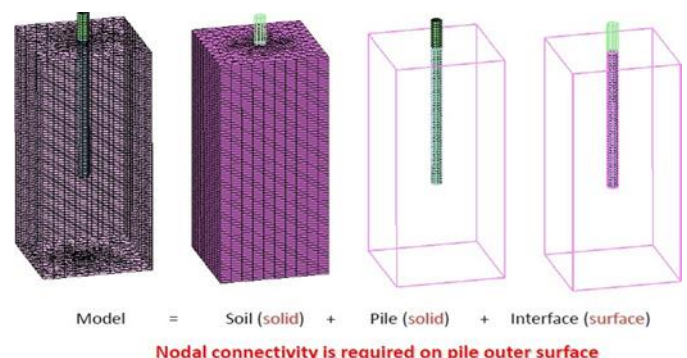
Fig. 3. Shcematic of a 3D model of pile with solid components. If it's required to think about the displacement between pile and soil and a discount in touch resistance between pile and soil in these models, surface interface components as its shown in Figure four will be used for connecting solid components.
