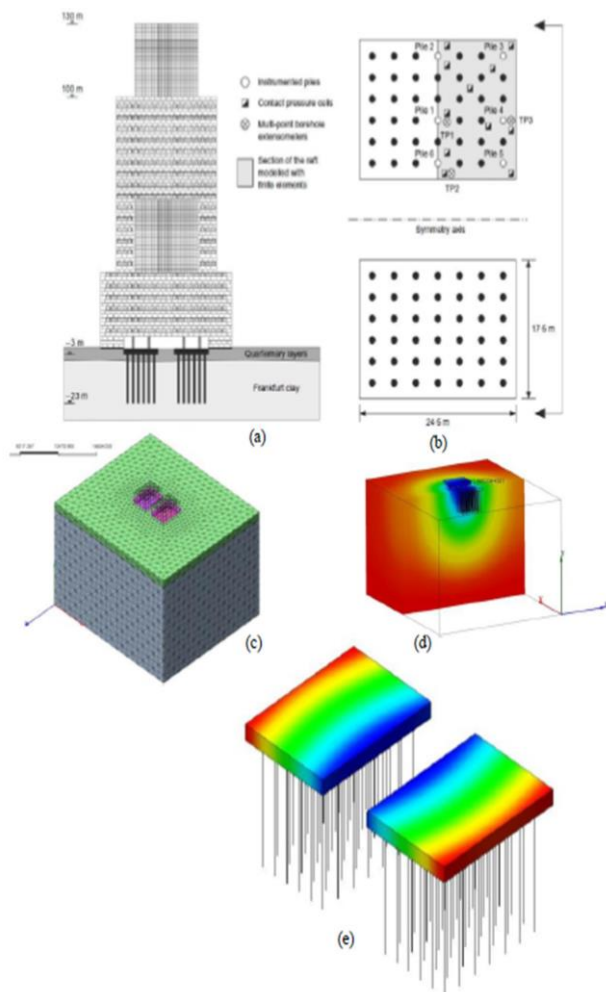
Fig. 17. (a), (b) Geometry details for Torhaus tower[26] (c), (d) and (e) validation process and result for Torhaus tower in MIDAS GTS software.
