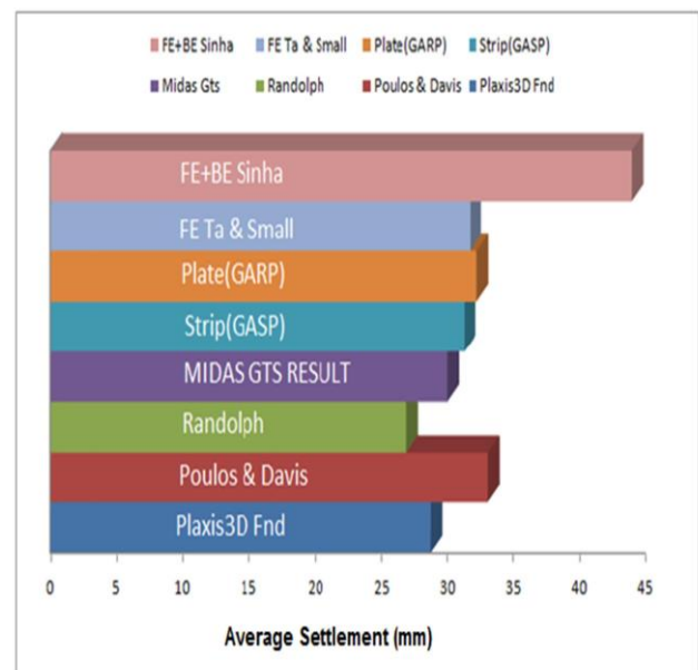
Fig. 16. Comparison of the results calculated using methods with calculated average settlement in MIDAS GTS for Poulos's hypothetical problem.
