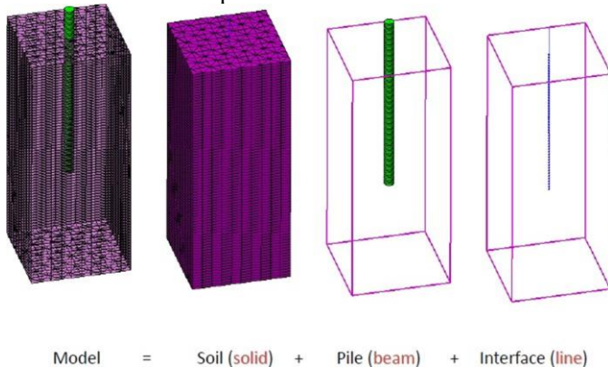
Fig. 5. Schematic of 3D model of the pile with beam- solid property elements.
