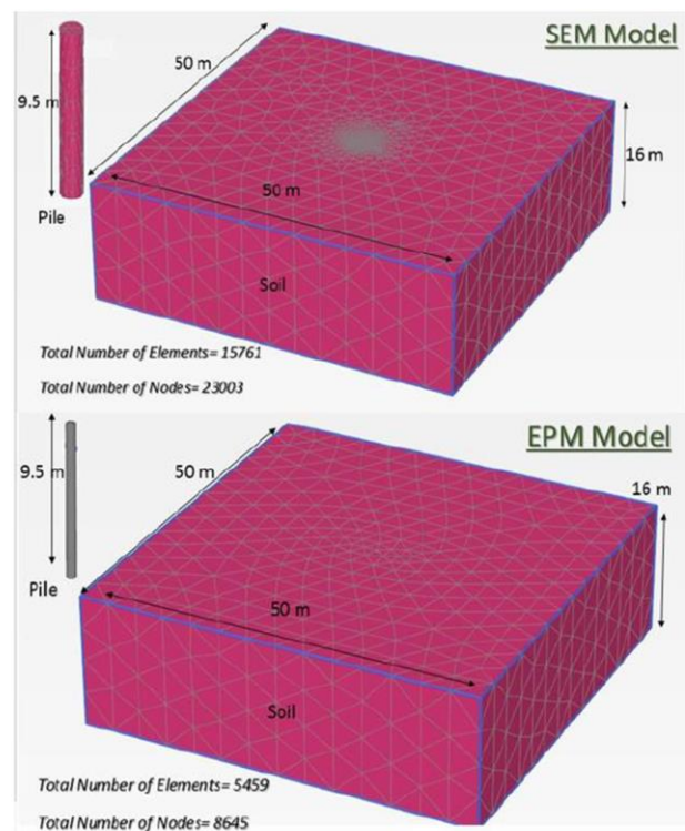
Fig. 12. Model properties for SEM and EPM models.
