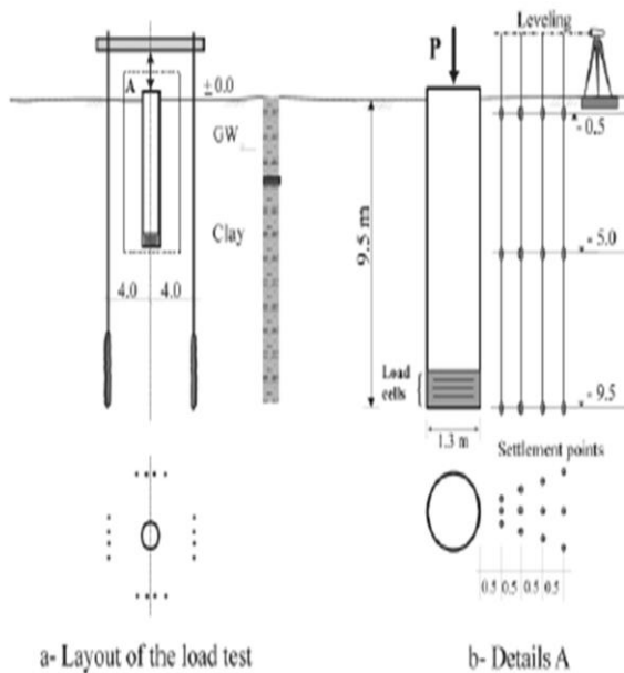
Fig. 10. Details of the pile loading test [15].
