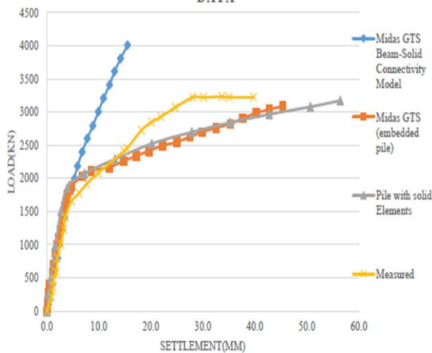
Fig. 13. A comparison between the pile's modeling techniques and test results.
