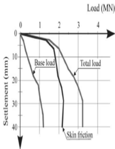
Fig. 11. Load-settlement curves for pile loading test [15].
