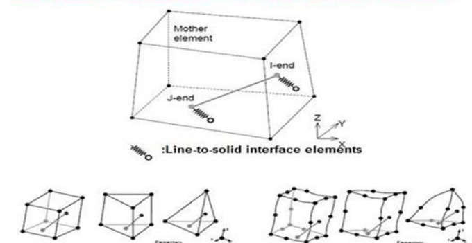
Fig. 5. Schematic of 3D model of the pile with beam- solid property elements.
