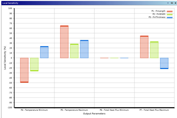
Figure 5.7: Local Sensitivity Bar Chart of Design of Experiments
