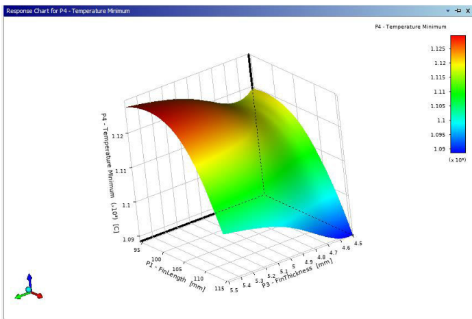
Figure 5.9: Response Surface (Fin Thickness Vs. Fin Length Vs. Minimum Temperature)
