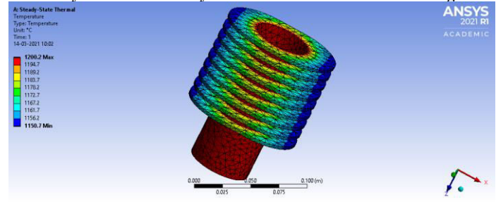
Figure 5.2: Temperature distribution plot of flat oval fins of an air cooled IC-engines
