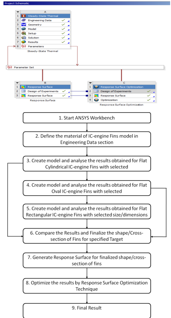
Figure 4.1: Methodology of the research
