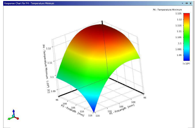
Figure 5.10: Response Surface (Fin Width Vs. Fin Length Vs. Minimum Temperature)
