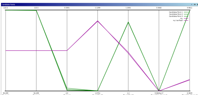
Figure 5.15: Candidate Point chart obtained from Response Surface optimization
