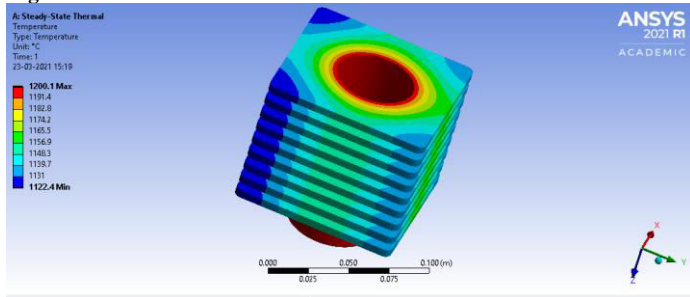
Figure 5.3: Temperature distribution plot of flat rectangular fins of an air cooled IC-engines
