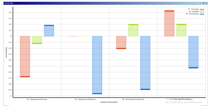
Figure 5.16: Sensitivity Chart generated by Response Surface Optimization
