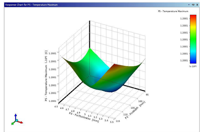
Figure 5.14: Response Surface (Fin Width Vs. Fin Thickness Vs. Maximum Temperature)
