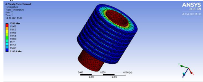
Figure 5.1: Temperature distribution plot of flat cylindrical fins of an air cooled IC-engines
