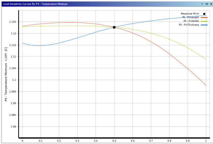
Figure 5.8: Local Sensitivity Curves of Design of Experiments
