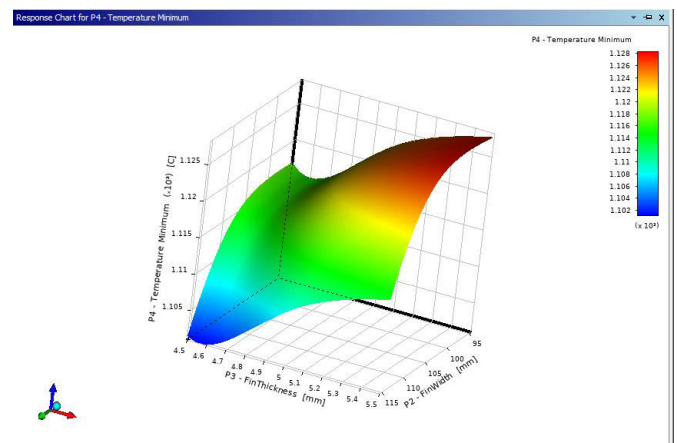
Figure 5.11: Response Surface (Fin Width Vs. Fin Thickness Vs. Minimum Temperature)
