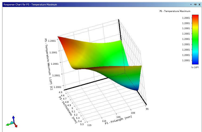
Figure 5.12: Response Surface (Fin Thickness Vs. Fin Length Vs. Maximum Temperature)
