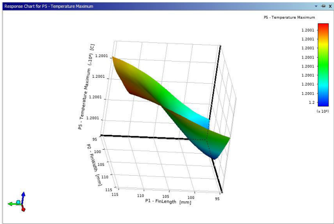
Figure 5.13: Response Surface (Fin Width Vs. Fin Length Vs. Maximum Temperature)
