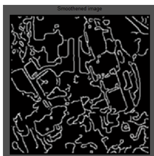
Fig 11 Smoothed Image
