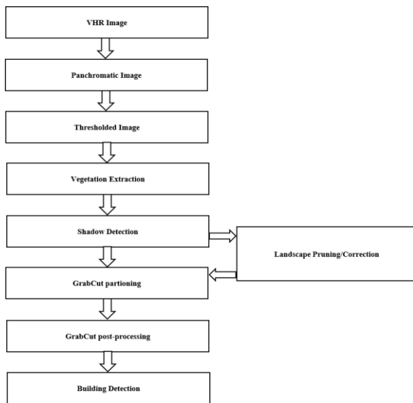
Fig 2. Building detection approach
