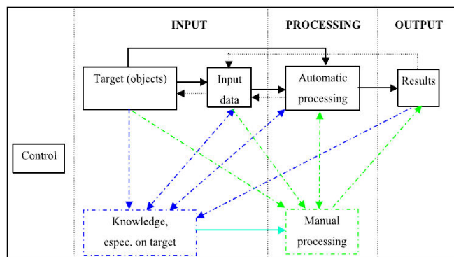
Fig 1. Architectures and components of image analysis systems for object extraction [7].
