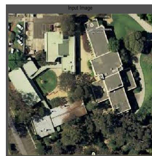
Fig 4 Input Image
