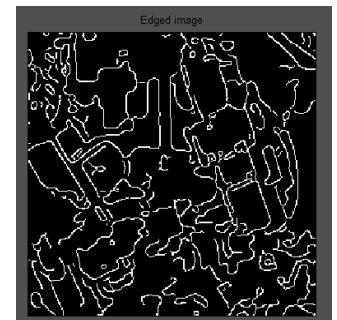
Fig 14 Edged Image
