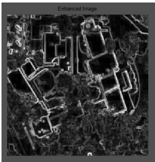
Fig 6 Enhanced Image
