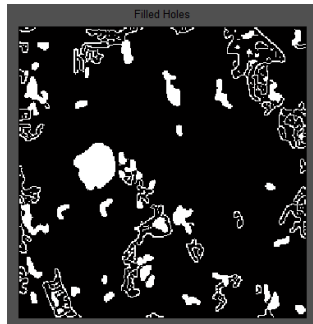
Fig 16 Filled Holes
