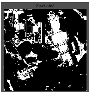
Fig 17 Dilated Image
