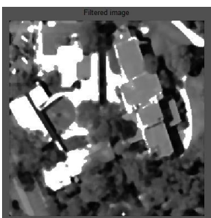
Fig 10 Filtered Image
