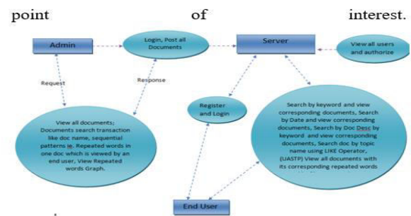
Figure 3: Data Flow Diagram
