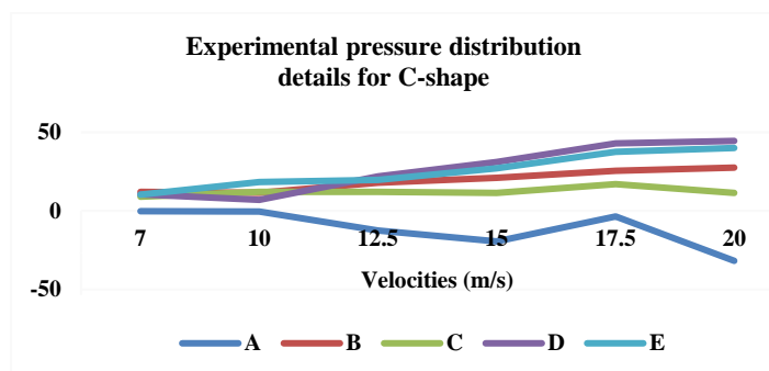
Figure no. 4 Velocity vs. Pressure distribution for C-Shape by experimental analysis
