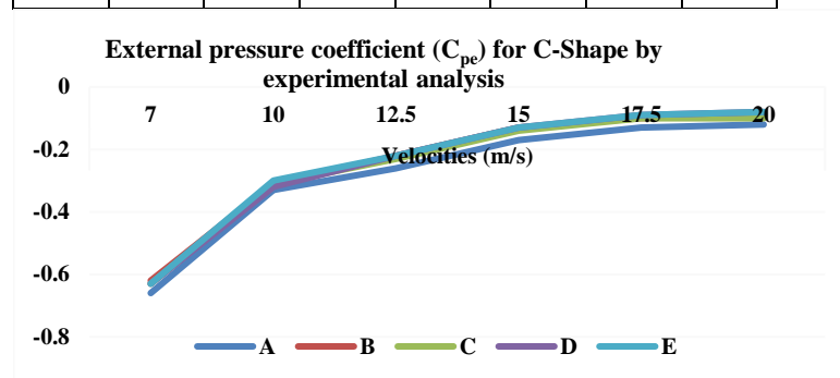
Figure 7 External pressure coefficient ( C_{pe} ) for C-Shape by experimental analysis
