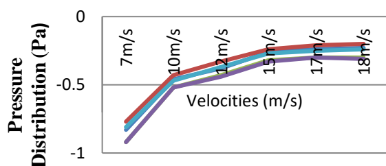
Velocity vs. Pressure distribution for L-Shape by software analysis
