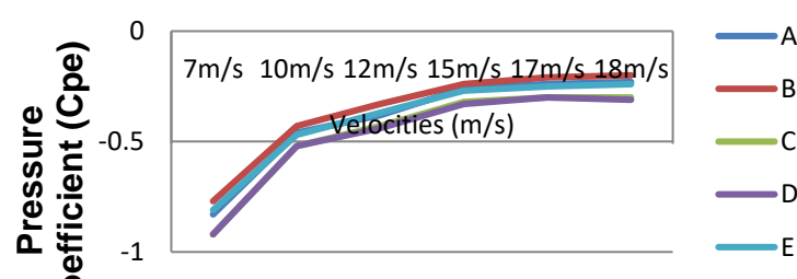
Figure 5 External pressure coefficient ( C_{pe} ) for L-Shape by experimental analysis
