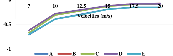
5 External pressure coefficient ( C_{pe} ) for I-Shape by experimental analysis
