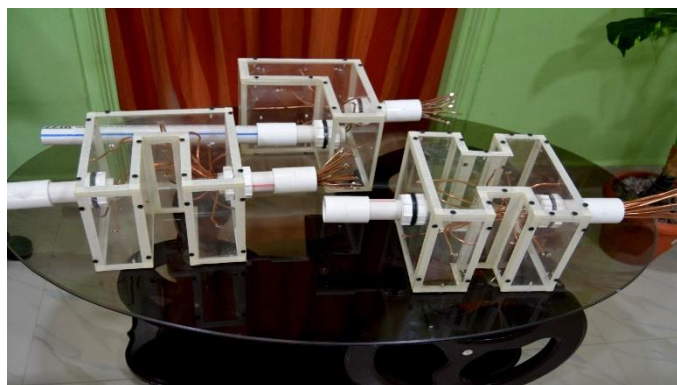
Figure 2 Acrylic models of C-Shape, I-Shape, L-Shape
