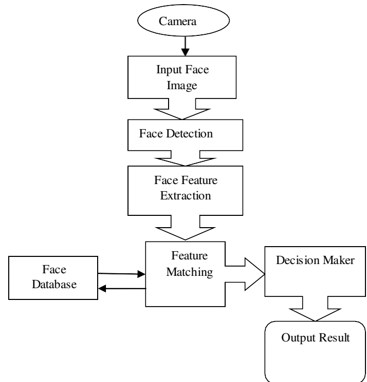
Fig 2.Work Flow Model
