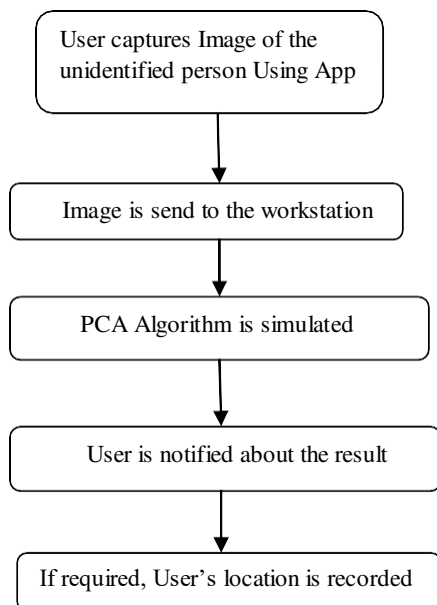
Fig.3 Workflow model
