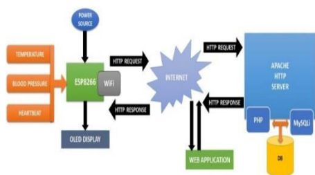
Fig 1. Block diagram of a patient health monitoring system
