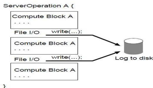
Figure 3.1: Scenario A has 10,000 processor-bound server operations where computation is interleaved with file write operations
