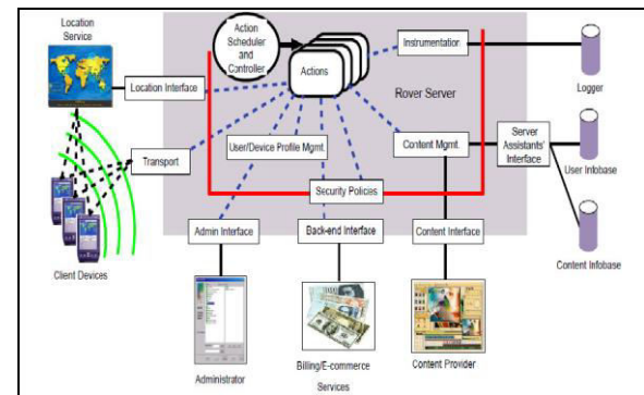
Figure 3.3: Logical architecture of a Rover system
