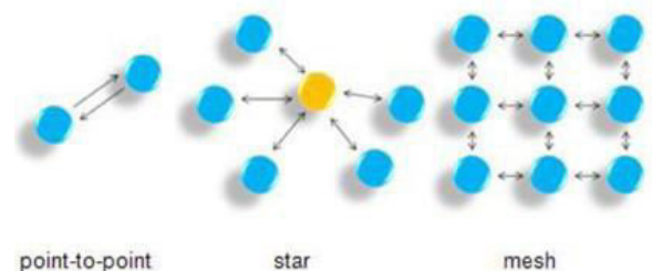
Figure 1.5. Basic wireless network topologies.
