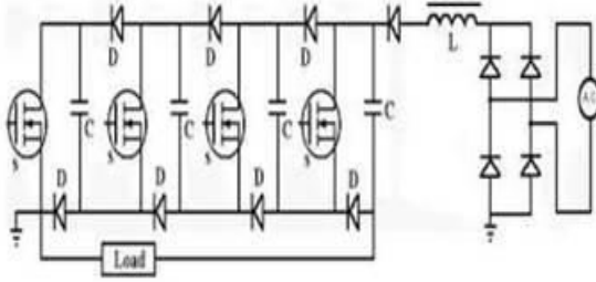
Fig.3 Modern Marx Generator
