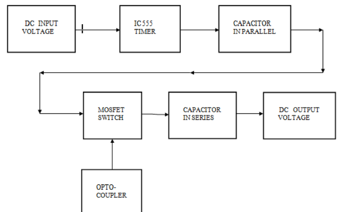
BLOCK DIGRAM
