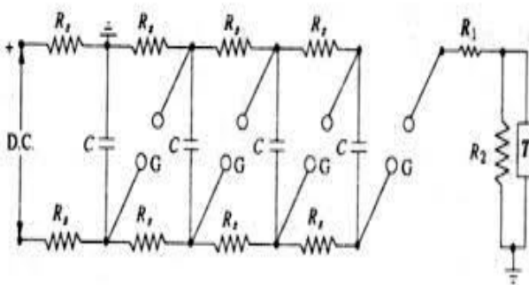
Fig. 2 Conventional Marx generator
