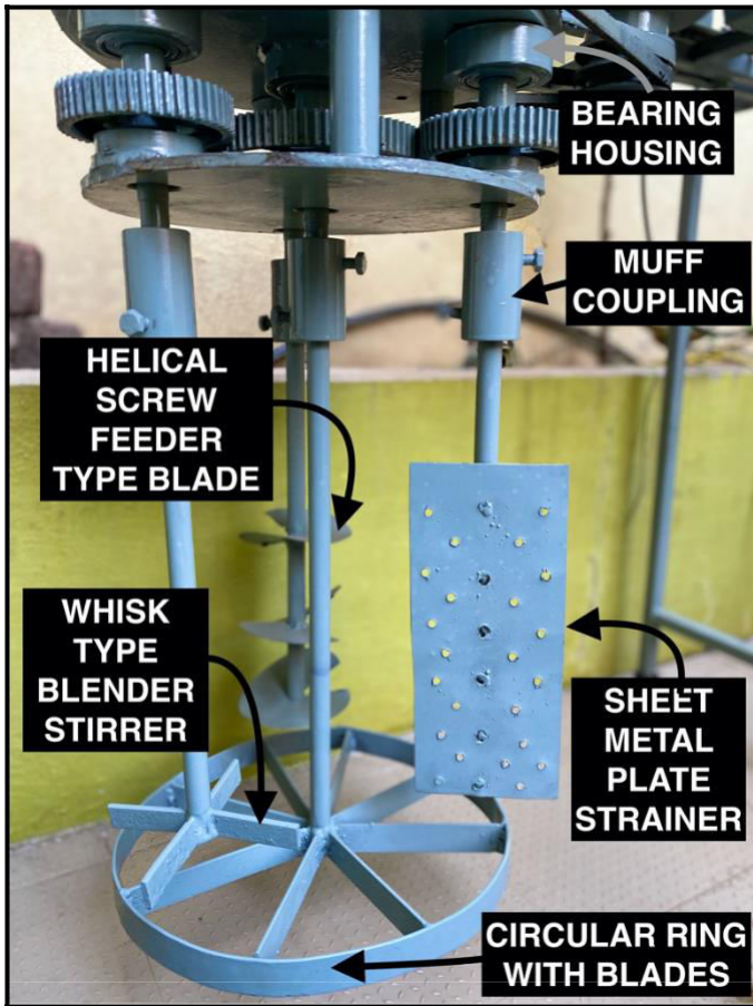
Fig. 3.2: Components.
