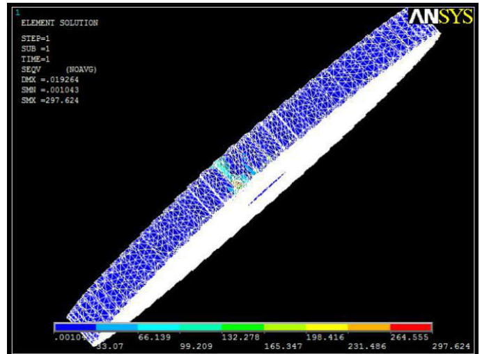
Fig. 5.1: Analysis of a spur gear stresses due to Radial Forces in ANSYS.
