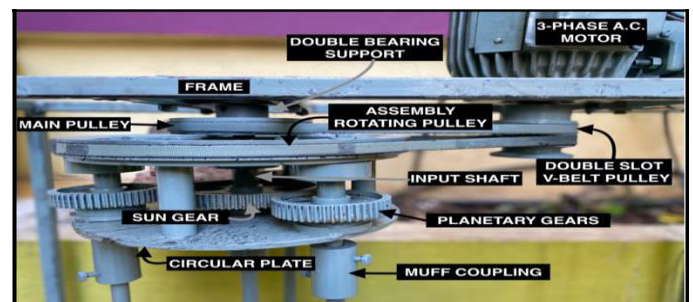
Fig. 3.1: Components.
