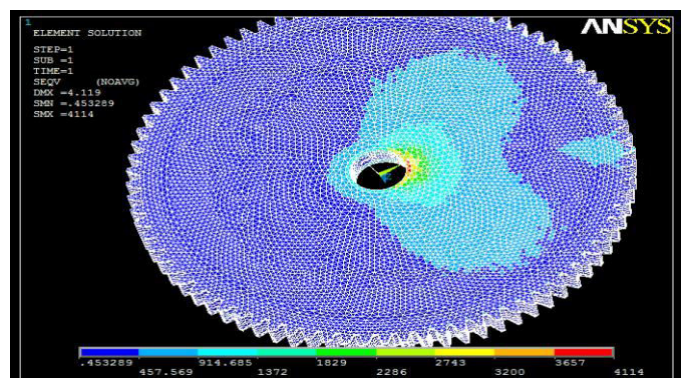
Fig. 5.2: Analysis of a Spur gear stresses due to Radial Forces in Radial Zoom.
