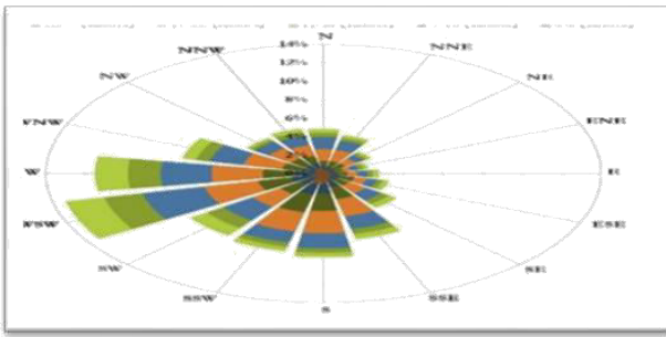
Fig.6. Windrose diagram for wind directions.
