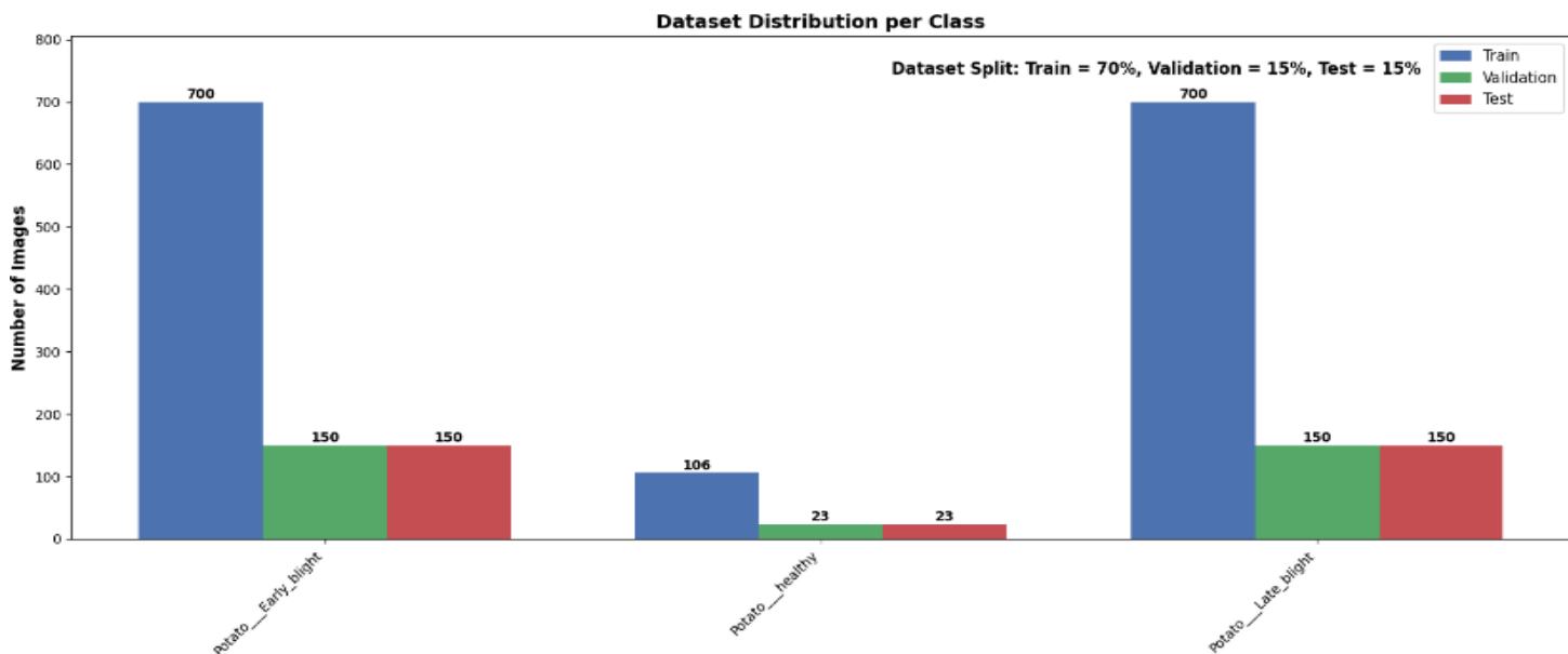
Figure 3: Data Splitting
