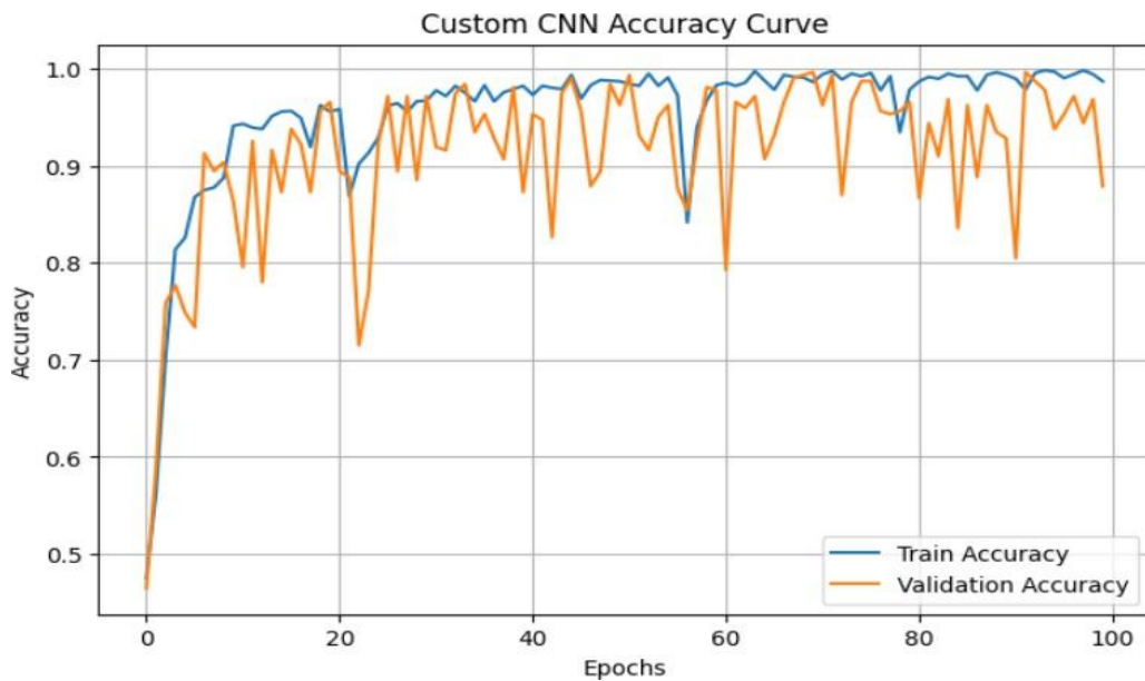
Figure 8: Training and Validation Accuracy over Epochs for Custom CNN Model
