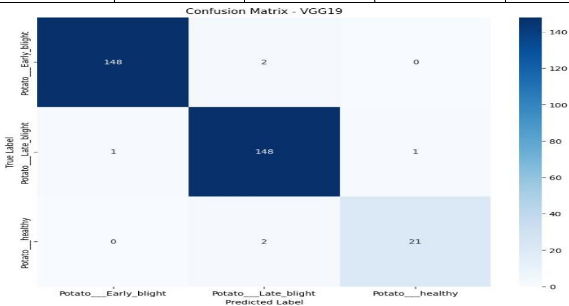
Figure 10: Confusion Matrix for VGG19
