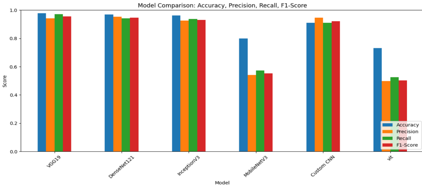
Figure 6: Bar Chart of Performance comparison of all models using Accuracy, Precision, Recall, and F1-score.
