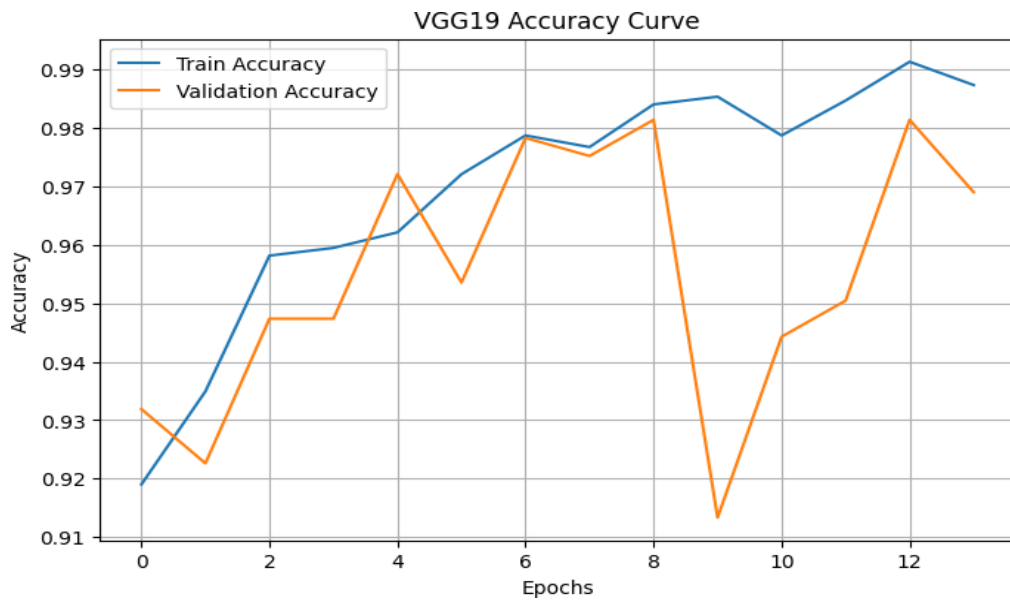
Figure 7: Training and Validation Accuracy over Epochs for VGG19 Model
