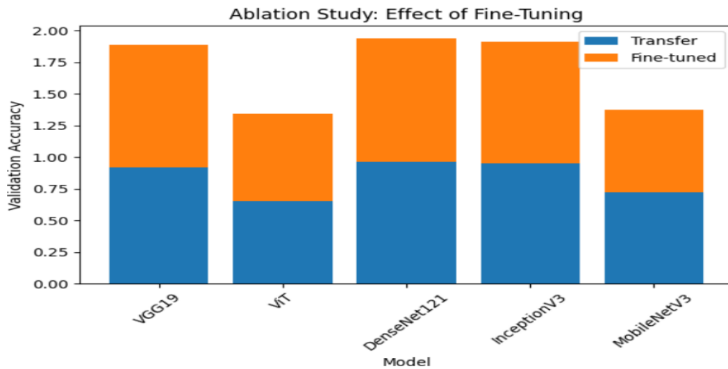
Figure 5: Impact of fine-tuning on validation accuracy across different models.
