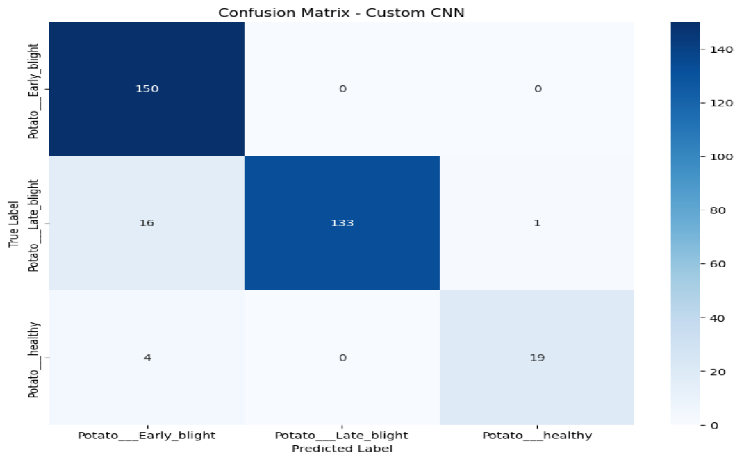
Figure 11: Confusion Matrix for Custom CNN
