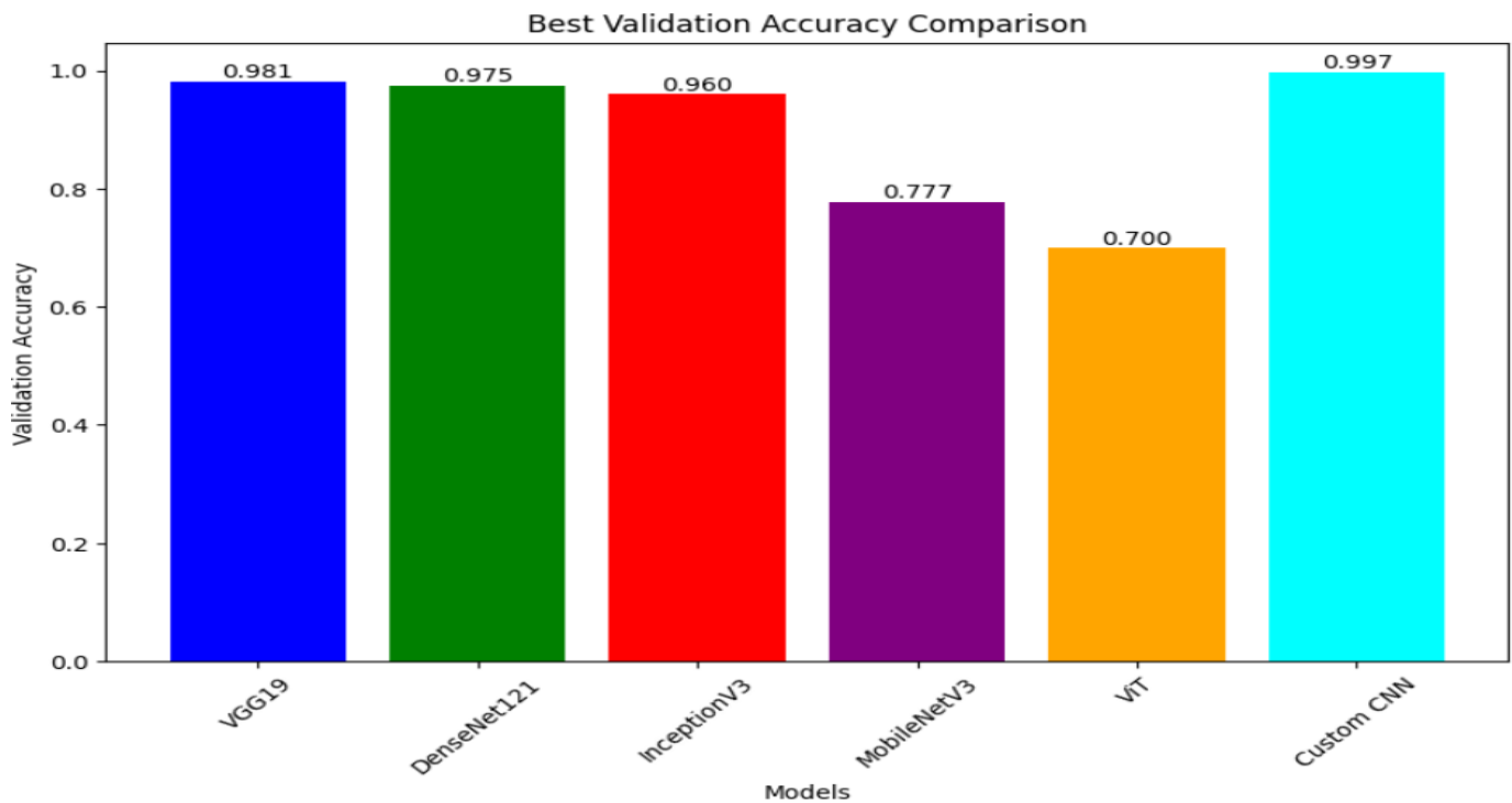
Figure 9: Bar Chart for Best Validation Accuracy for all models
