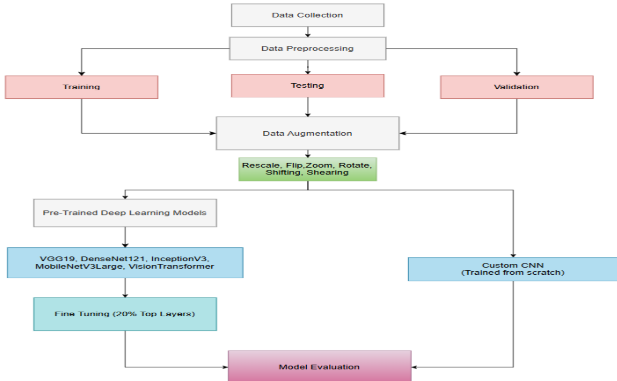
Figure 1: System Flowchart
