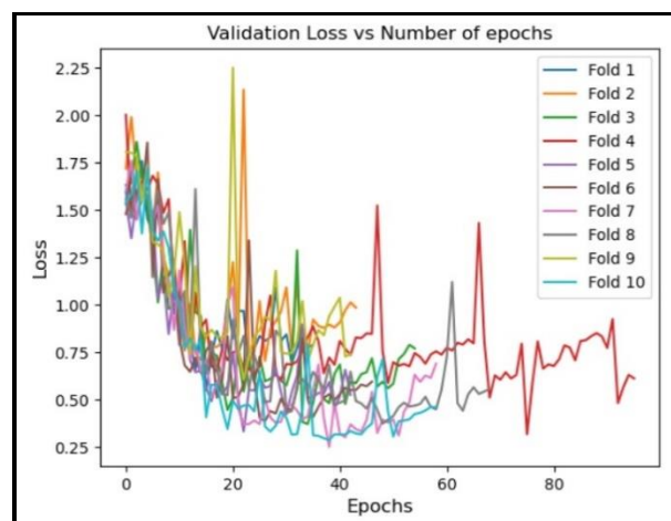
Figure 6. History of loss in the 10 folds.
