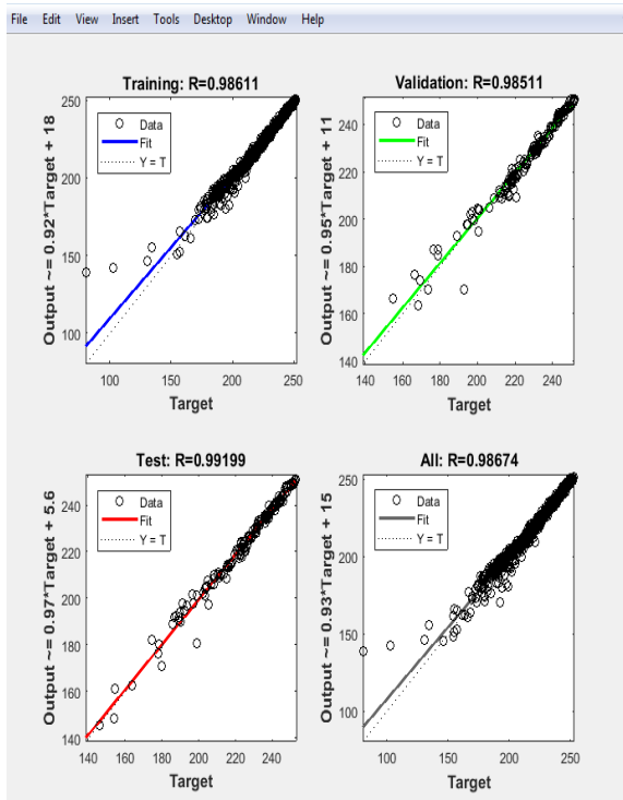
Fig.8 Regression Analysis
