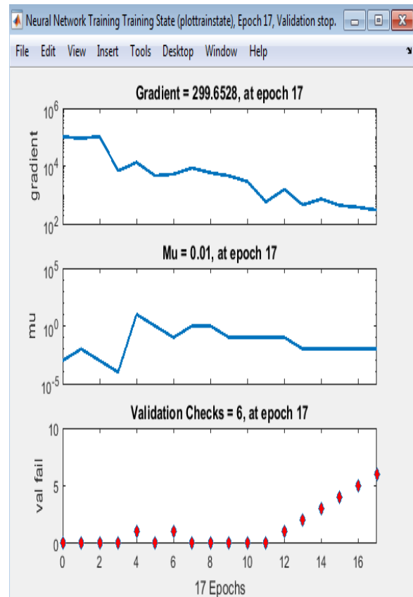
Fig.7 Training Parameters
