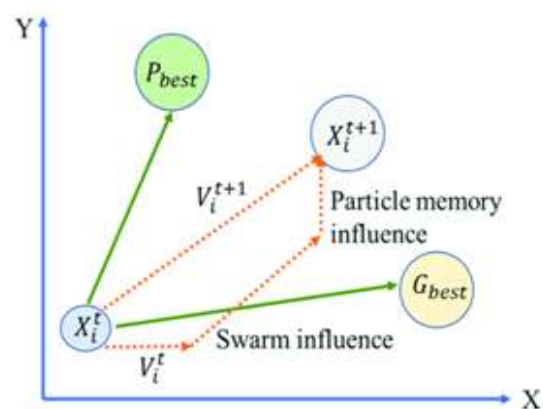
Fig.2 Visualization of PSO
