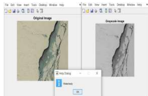
Fig.9 Object Detection
