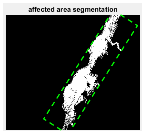
Fig.7 Segmentation
