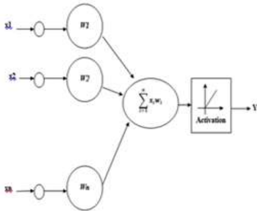
Fig.3 Mathematical Model of Neural Network
