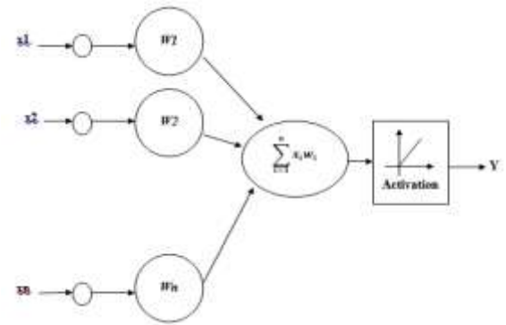
Fig.1 Mathematical Model of Neural Network
