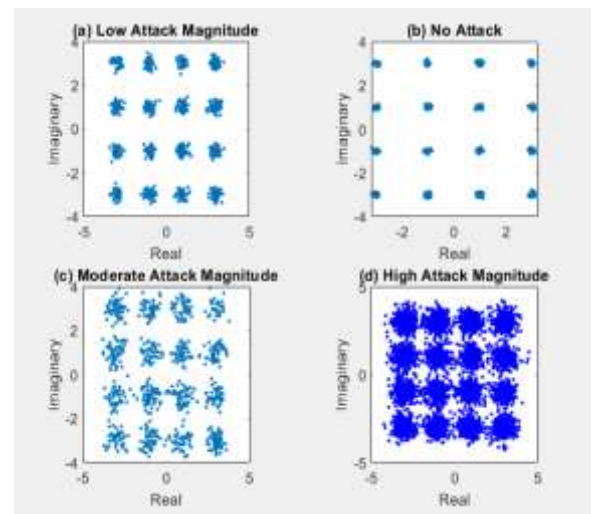
Fig.5 Scatter Plots
