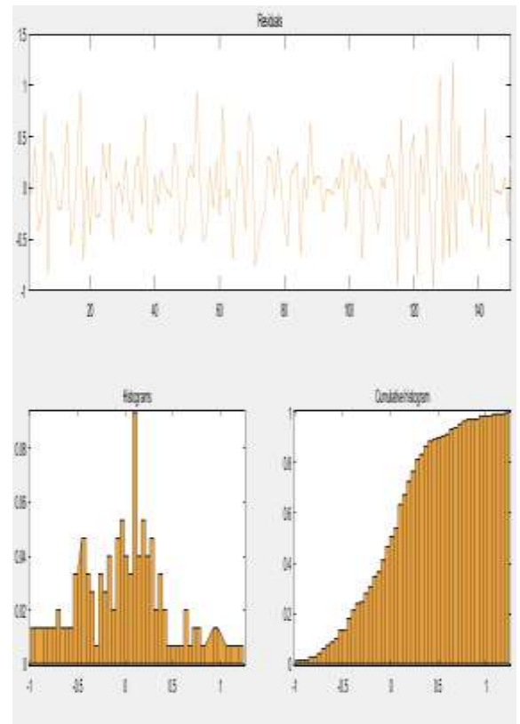
Fig. 7 Residual Histograms
