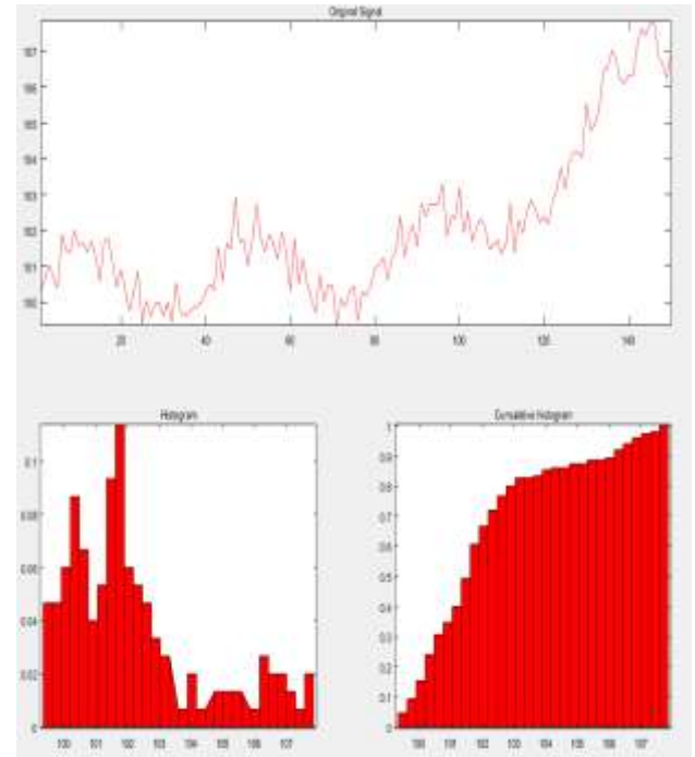
Fig. 4 Original Histogram
