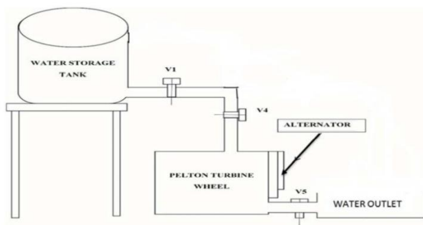
Figure 6. Hydro turbine setup.
