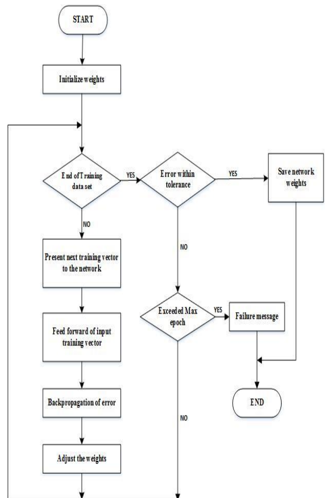
Fig.3 Flowchart of Back Propagation
