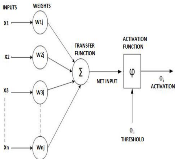
Fig.2 Mathematical Modeling of ANN
