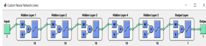
Fig.4 Designed Model
