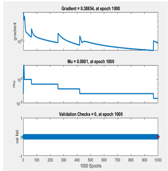
Fig.6 Training Parameters
