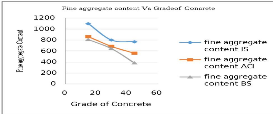
Figure 4 Fine aggregate content Vs. Grade of Concrete
