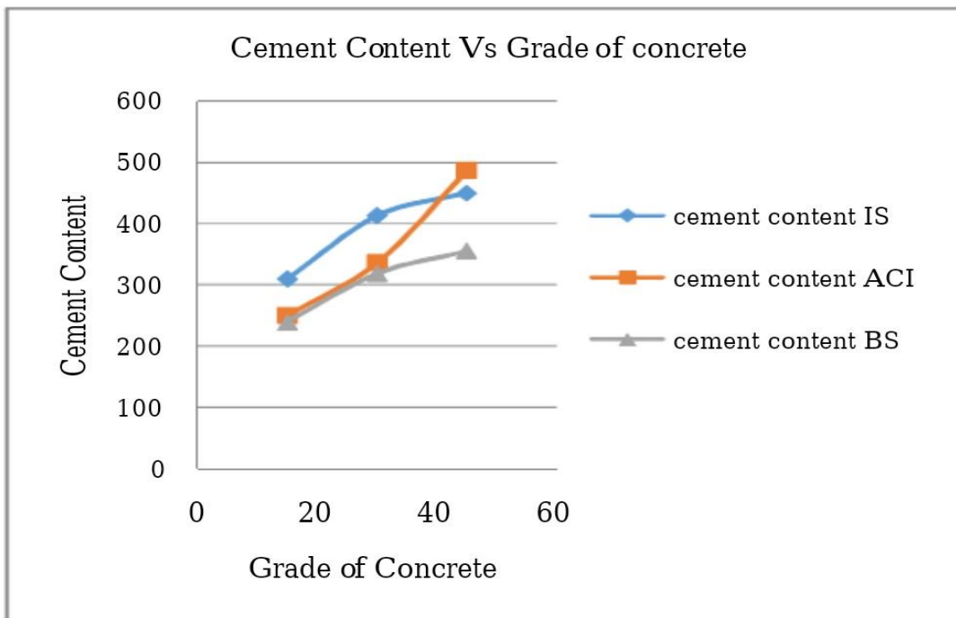
Figure 3 Cement Content Vs. Grade of Concrete
