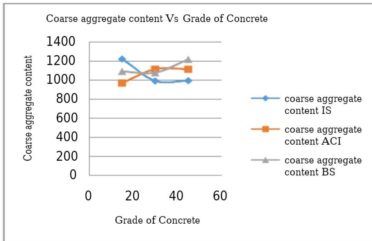
Figure coarse aggregate content Vs. Grade of Concrete
