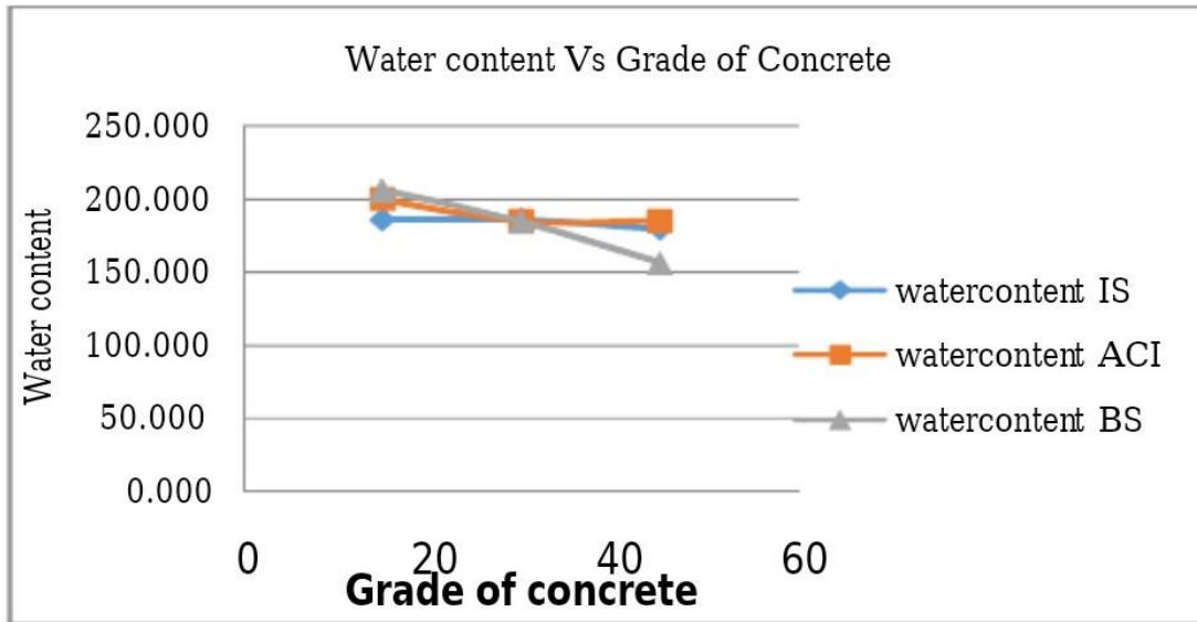
Figure 2 Water content Vs. Grade of Concrete
