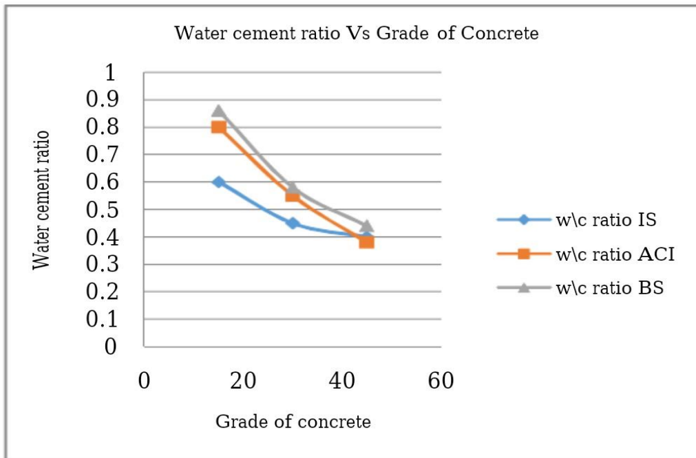
Figure 1 Water cement ratio Vs. Grade of Concrete
