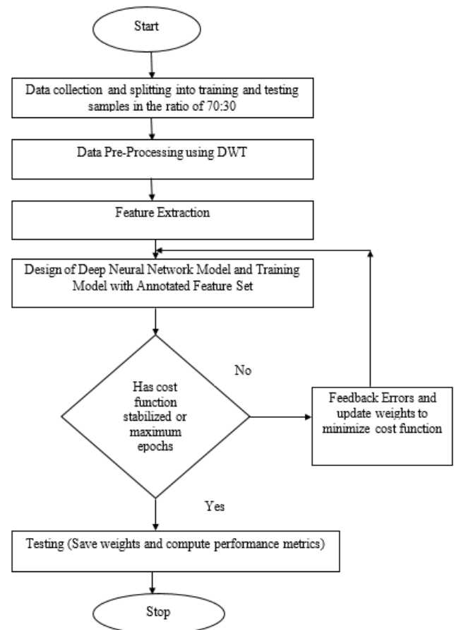
Fig.3 Flowchart of Proposed System
