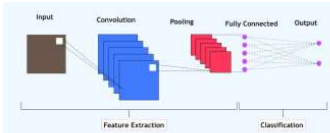
Fig.2 The CNN Model
