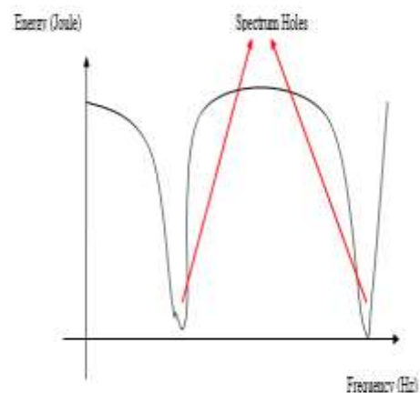
Fig.2 Energy Detection
