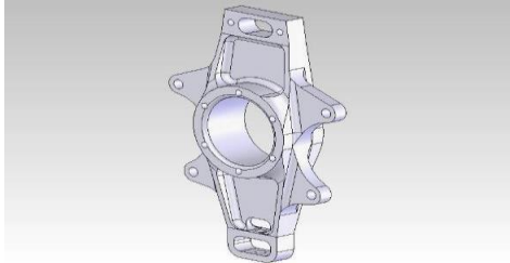
Fig.1 4. Upright of formula student vehicle
