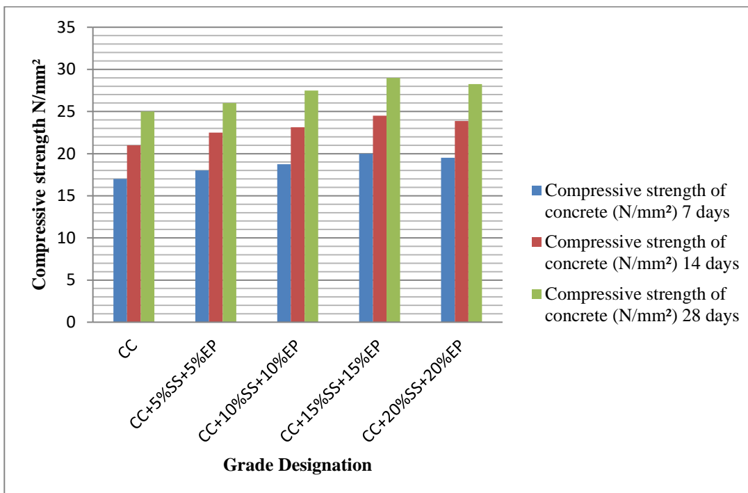
Graph:1 Compressive Strength of concrete for 7days,14days,28days
