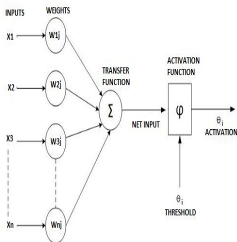
Fig.3 Mathematical Modeling of ANN
