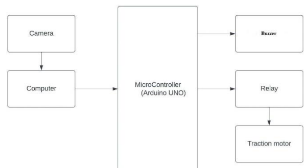
Fig.1: Block Diagram
