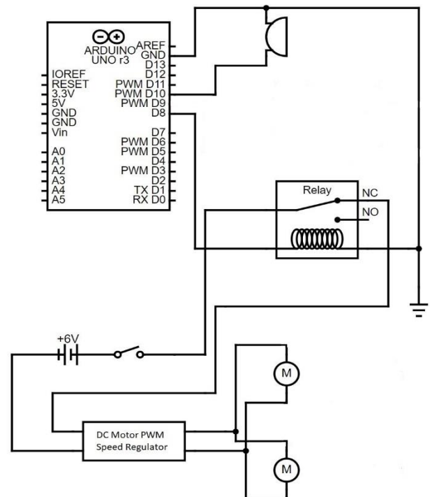
Fig.2: Circuit diagram
