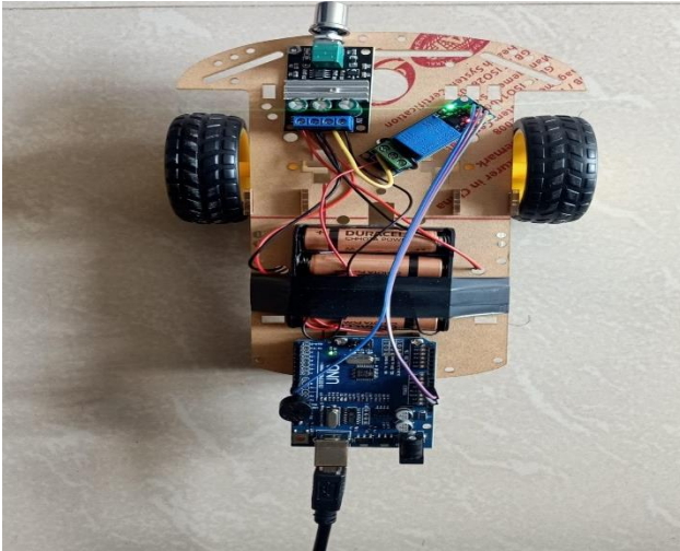
Fig.3: Prototype Image
