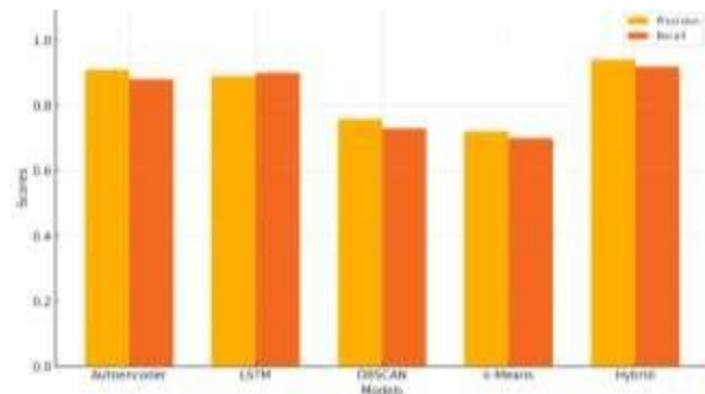
Figure 2: Precision and Recall Comparison of AI Models for Anomaly Detection in 5G Core and RAN
