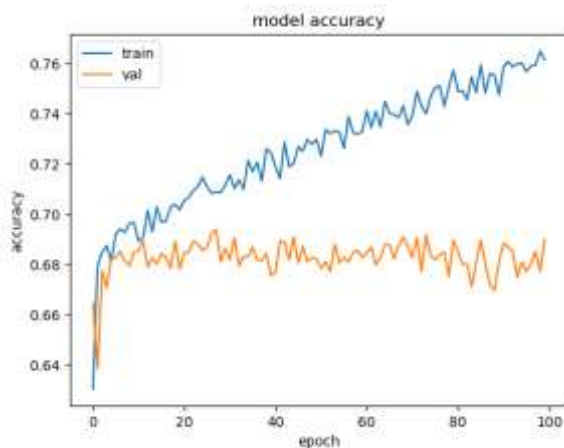
Figure 3. Model accuracy
