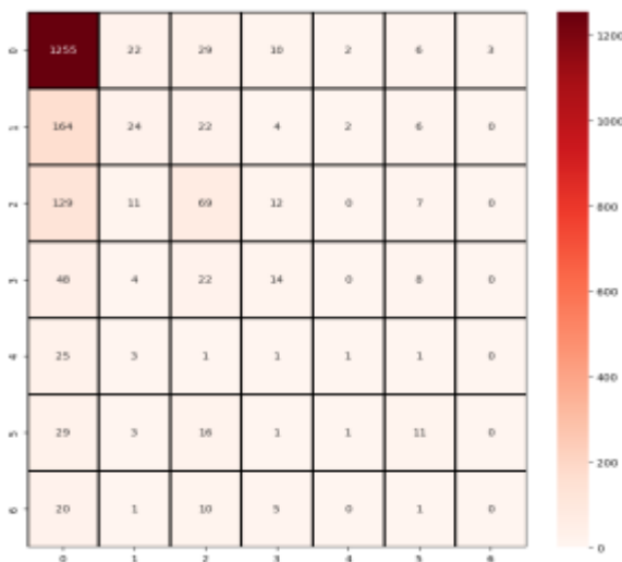
Figure 4. Classification Report
