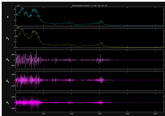
Fig.4 Haar Decomposition at Level 3
