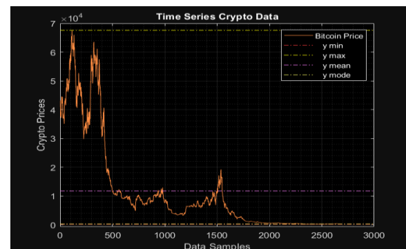
Fig.3 Original Bitcoin Price
