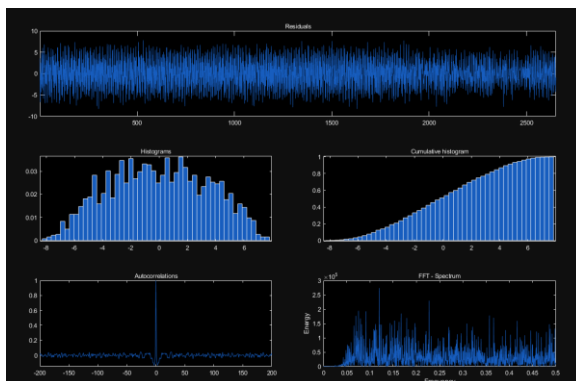
Fig.6 Multi-Resolution Analysis
