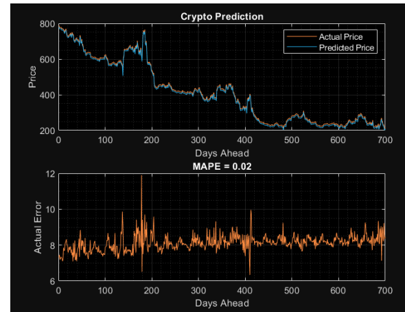
Fig.7 Predicted and Actual Crypto Behavior
