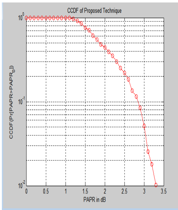
Fig.10 CCDF of proposed scheme
