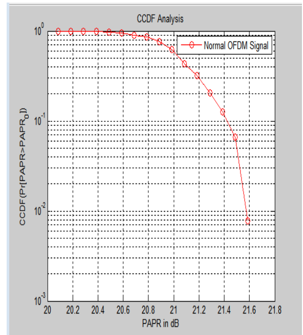
Fig.8 CCDF of original OFDM
