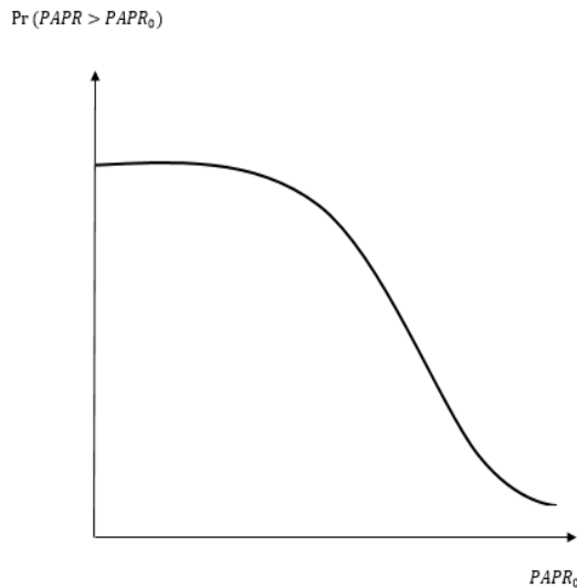
Fig.4 Typical PAPR CCDF graph for OFDM systems
