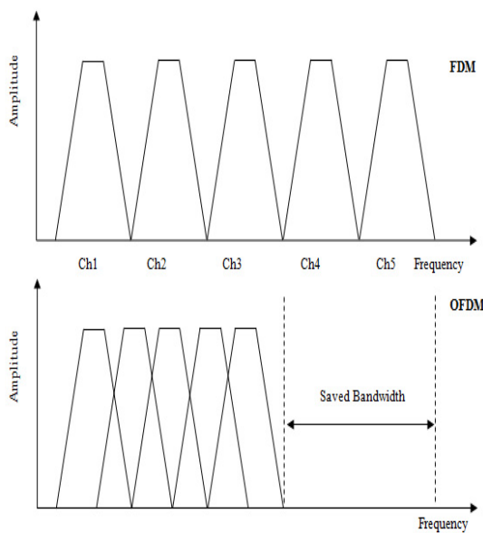
Fig.2 Graphical condition for orthogonality
