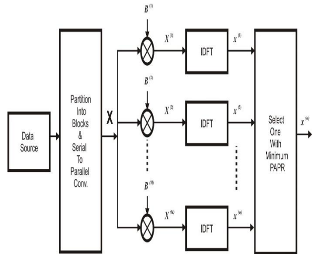
Fig.5 Block diagram for SLM
