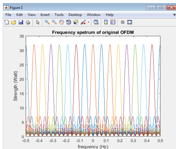
Fig.7 Spectrum of OFDM
