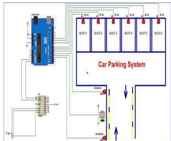
Fig. 4. Schematic Design of Automatic Parking system. Witness the intricate and visionary schematic diagram, showcasing a sequential implementation of all components in our remarkable project. [1]
