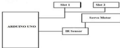
Fig. 5. Entry point basic diagram.
