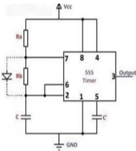
Fig. 1. IC 555 in the Astable Mode.
