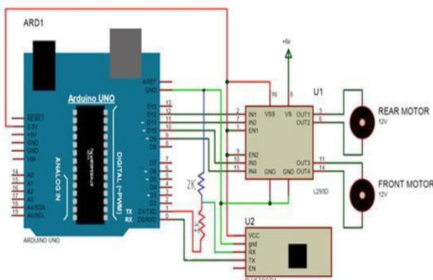
Figure 2: Robotic Vehicle Circuit using Arduino UNO
