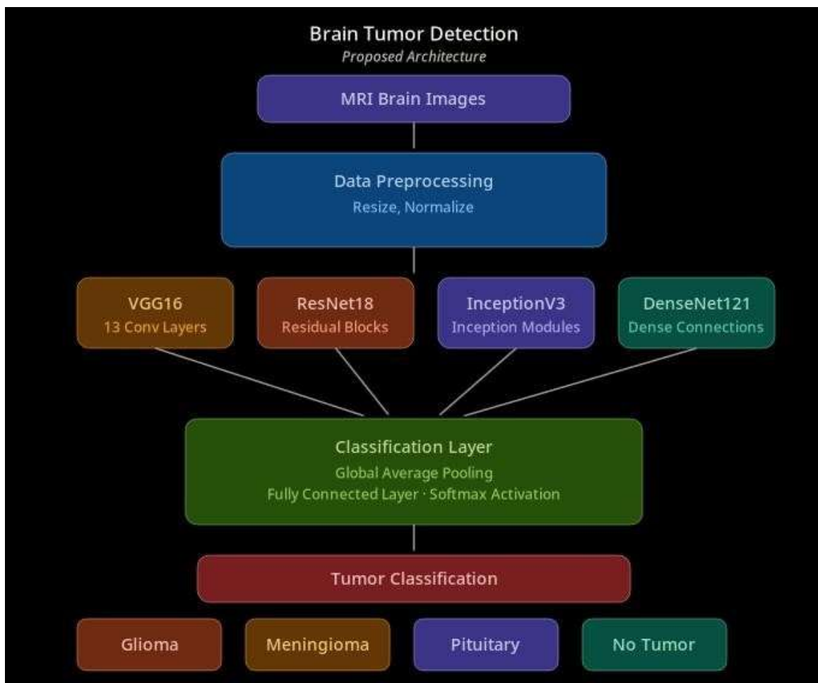
Fig:3.1: Brain tumor detection using Deep Learning Models
