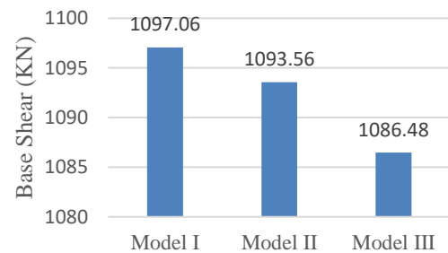
Graph -1: Base shear for static equivalent analysis.
