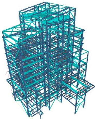
Fig -2: 3D View of Model II
