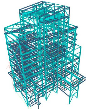
Fig -3: 3D View of Model III
