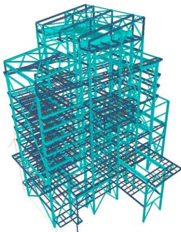
Fig -1: 3D View of Model I
