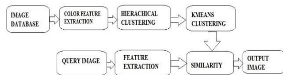
Figure 1: Block Diagram of Content Based Image Retrieval
