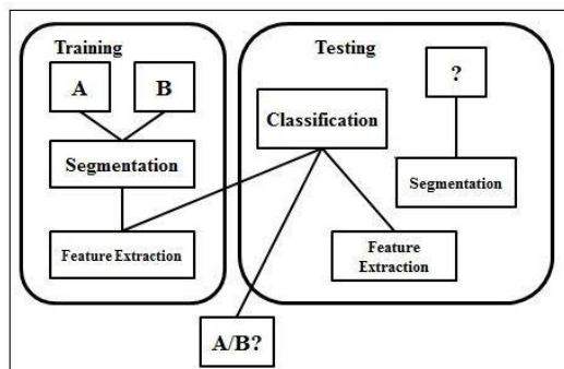
Fig.4. Classification Process
