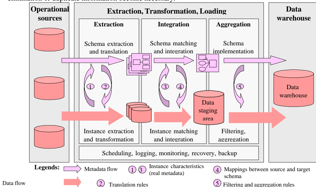
Figure 1. Steps of building a data warehouse: the ETL process
