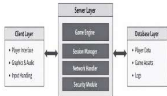
Fig. 1. System Architecture of Death Mania Multiplayer Game.
