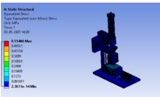
Fig. 9. Equivalent Stress
