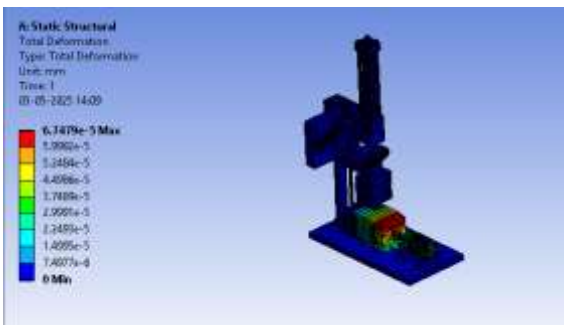
Fig. 8. Total Deformation
