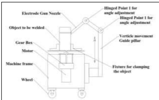
Fig. 2: 2d layout of required SPM
