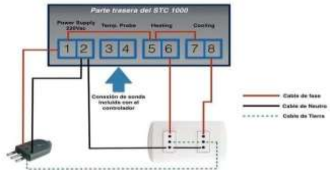
Fig – 5. Connections of STC 1000 Temperature
