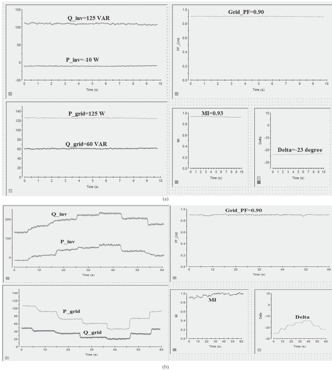
Fig. 14. System parameters where the inverter is connected to the grid. (a) When wind speed is zero and there is no active power coming from wind emulator. (b) When wind speed is changing and the incoming active power from the wind emulator is changing.
