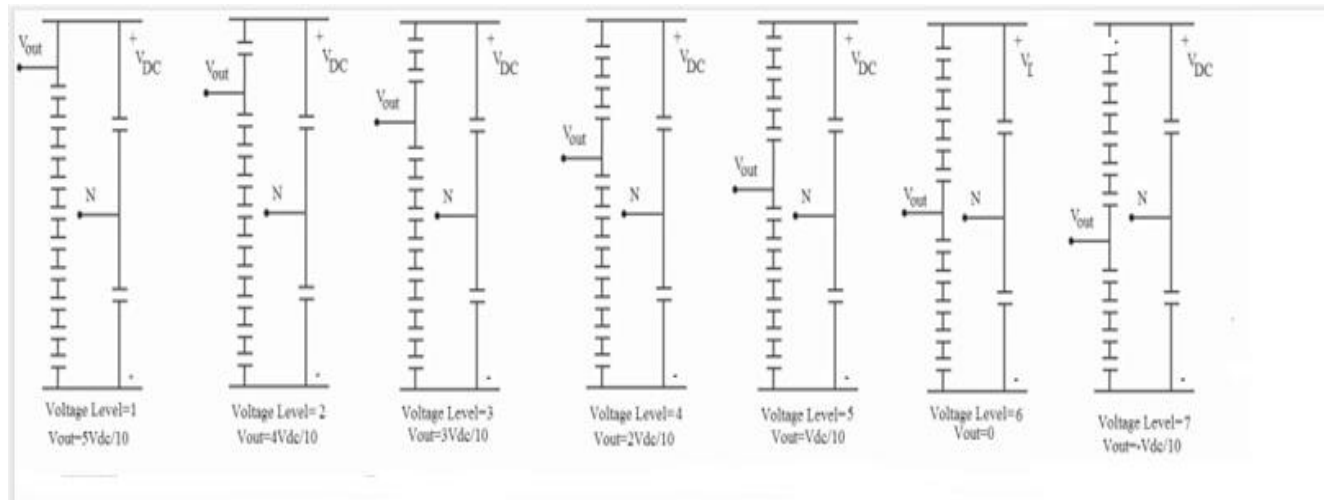
Fig. 5. Selection of SMs' capacitors for different voltage levels.
