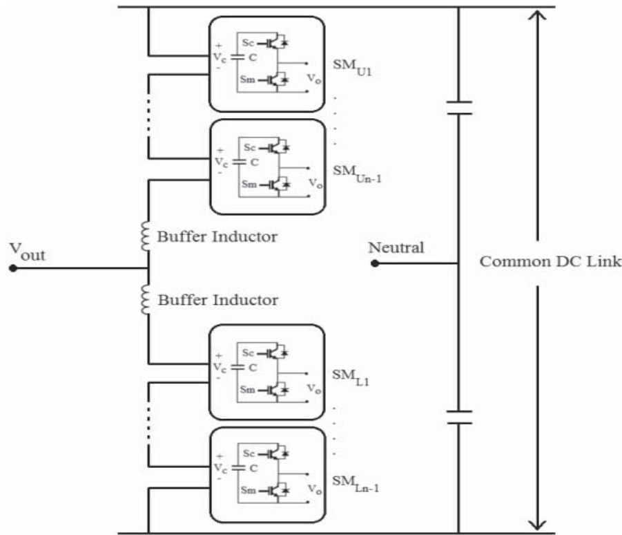
Fig. 2. Structure of a single-phase MMC inverter structure.
