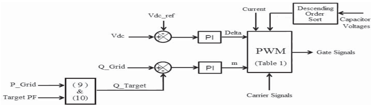
Fig. 3. Schematic of the proposed controller system.
