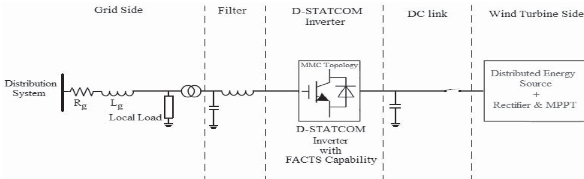
Fig. 1. Complete configuration of the proposed inverter with FACTS capability.
