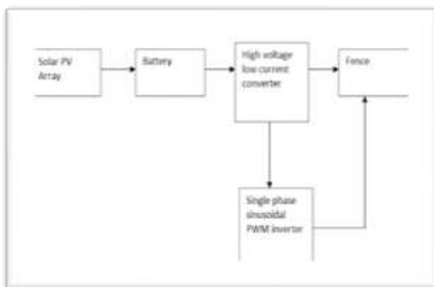
fig 2: block diagram
