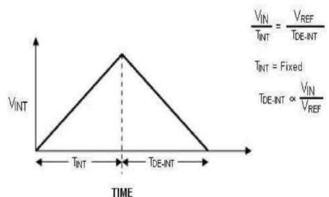
Fig 1: Dual Slope ADC
