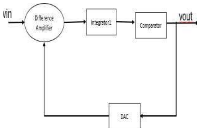
Fig 5: Second order sigma delta modulator
