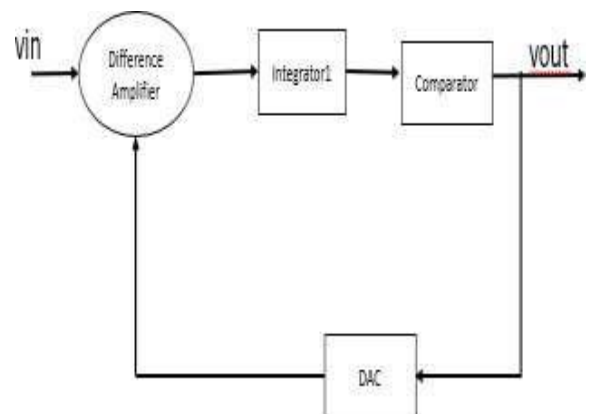
Fig 6: Second order sigma delta modulator
