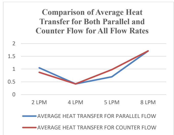
Graph 6 Comparison of Average Heat Transfer for Both Parallel and Counter Flow for All Flow Rates
