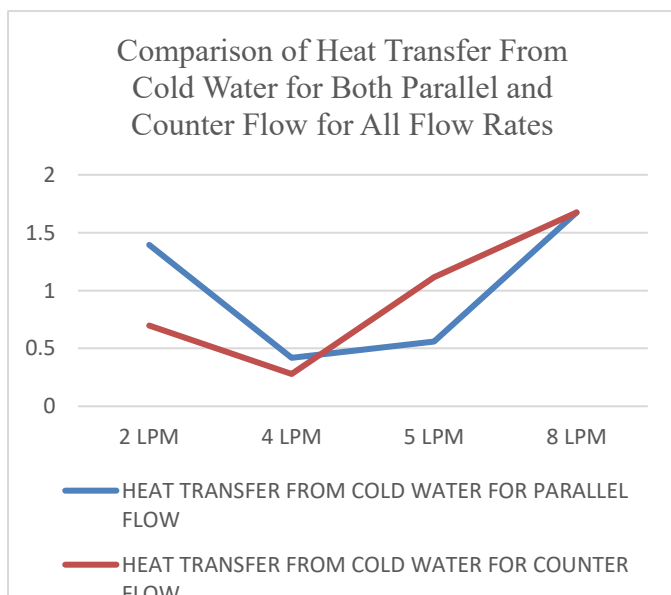
Graph 5 Comparison of Heat Transfer from Cold Water for Both Parallel and Counter Flow for All Flow Rates
