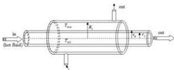
Fig. 3.1 Schematic Diagram of Tube in Tube Heat Exchanger 3.1 Working Principle
