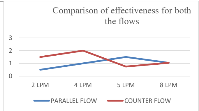
Graph 2 Comparison of Effectiveness for Both Parallel and Counter Flow for All Flow Rates
