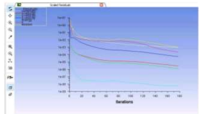
Fig.7 Scale Residual
