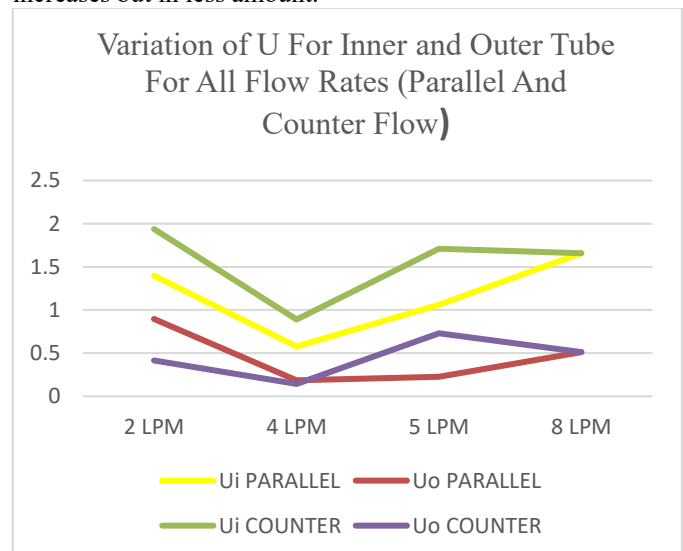
Graph 3 Variation of U For Inner and Outer Tube for All Flow Rates (Parallel and Counter Flow)
