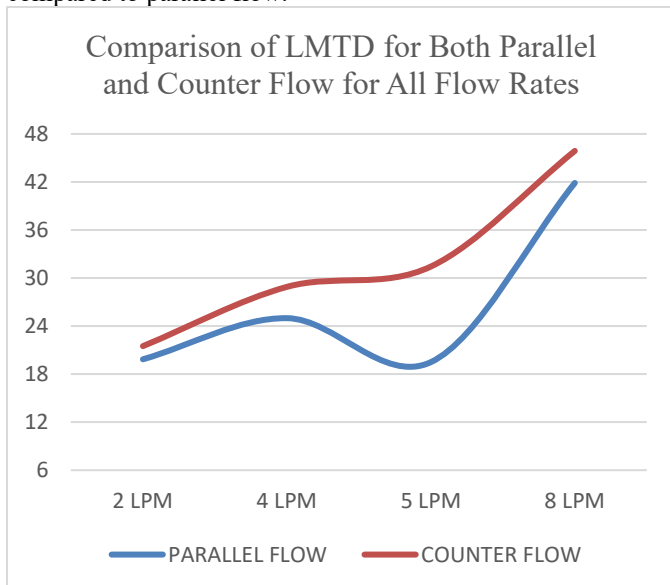
Graph. 1 Comparison of LMTD for Both Parallel and Counter Flow for All Flow Rates
