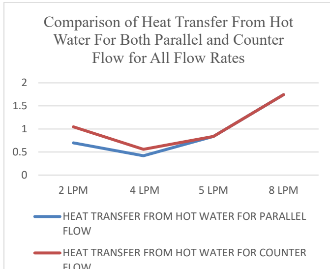
Graph 4 Comparison of Heat Transfer from Hot Water for Both Parallel and Counter Flow for All Flow Rates
