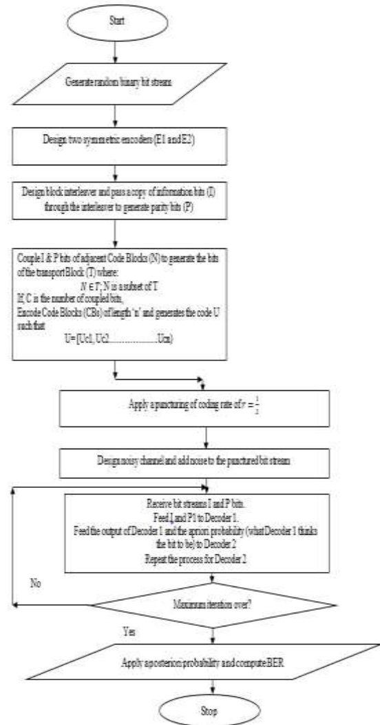
Fig.8 Proposed Flowchart
